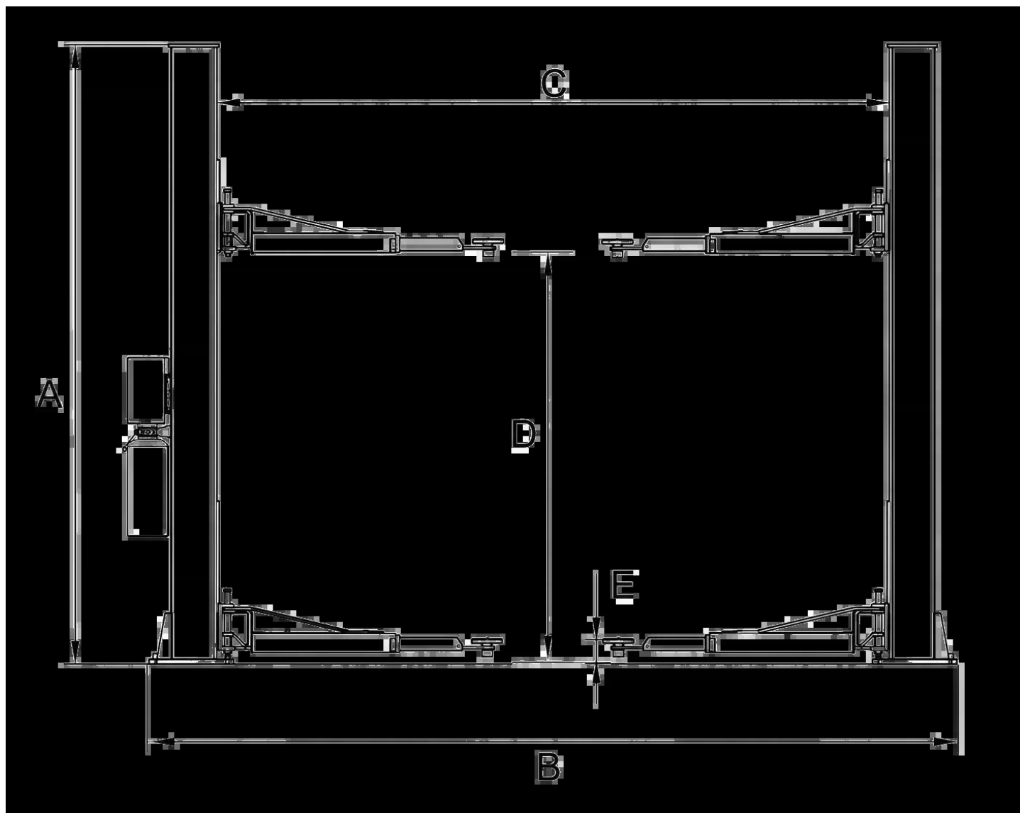
Lift Dimensional Diagram
