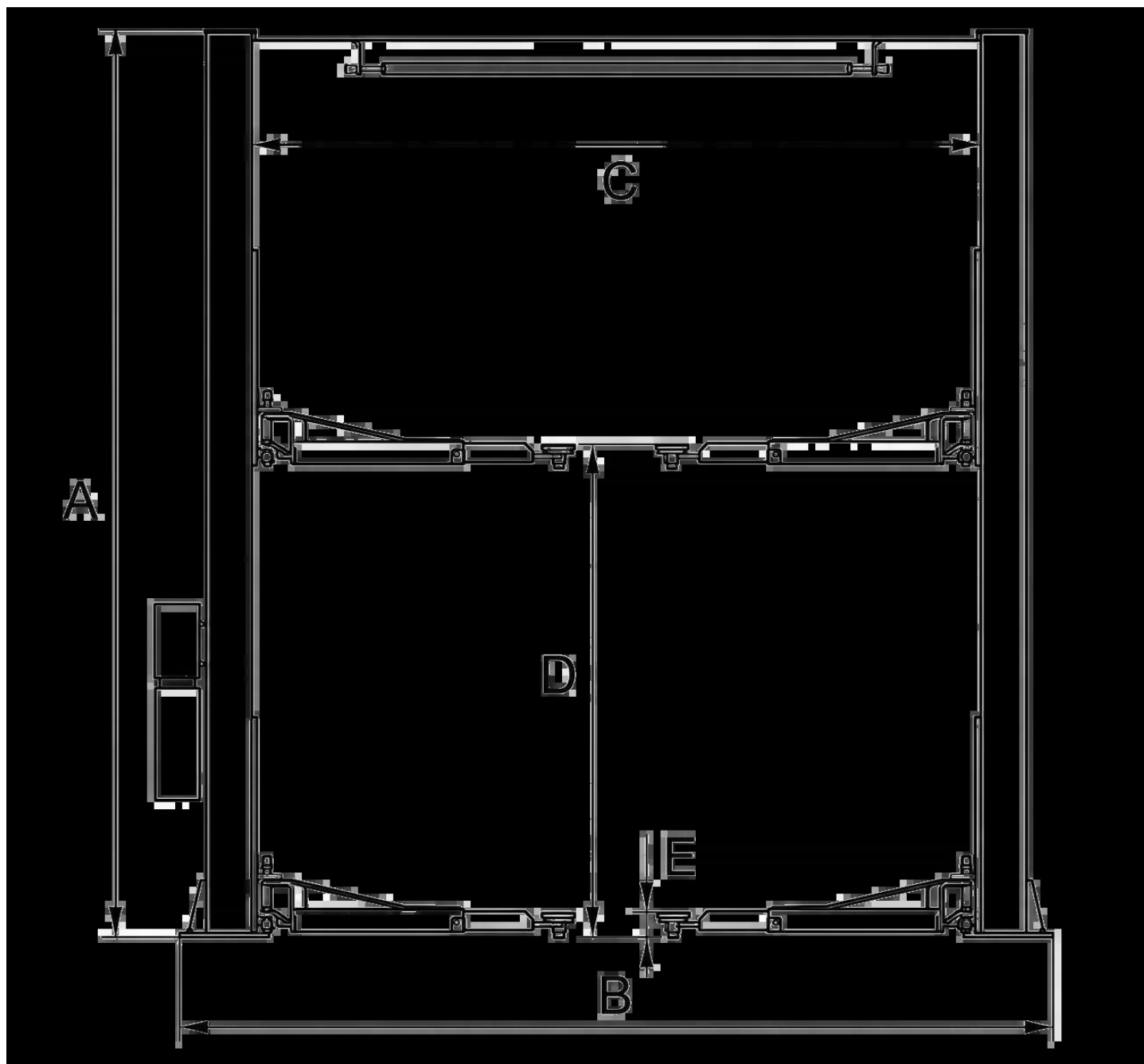
Overhead-Beam Lift Dimensional Diagram
